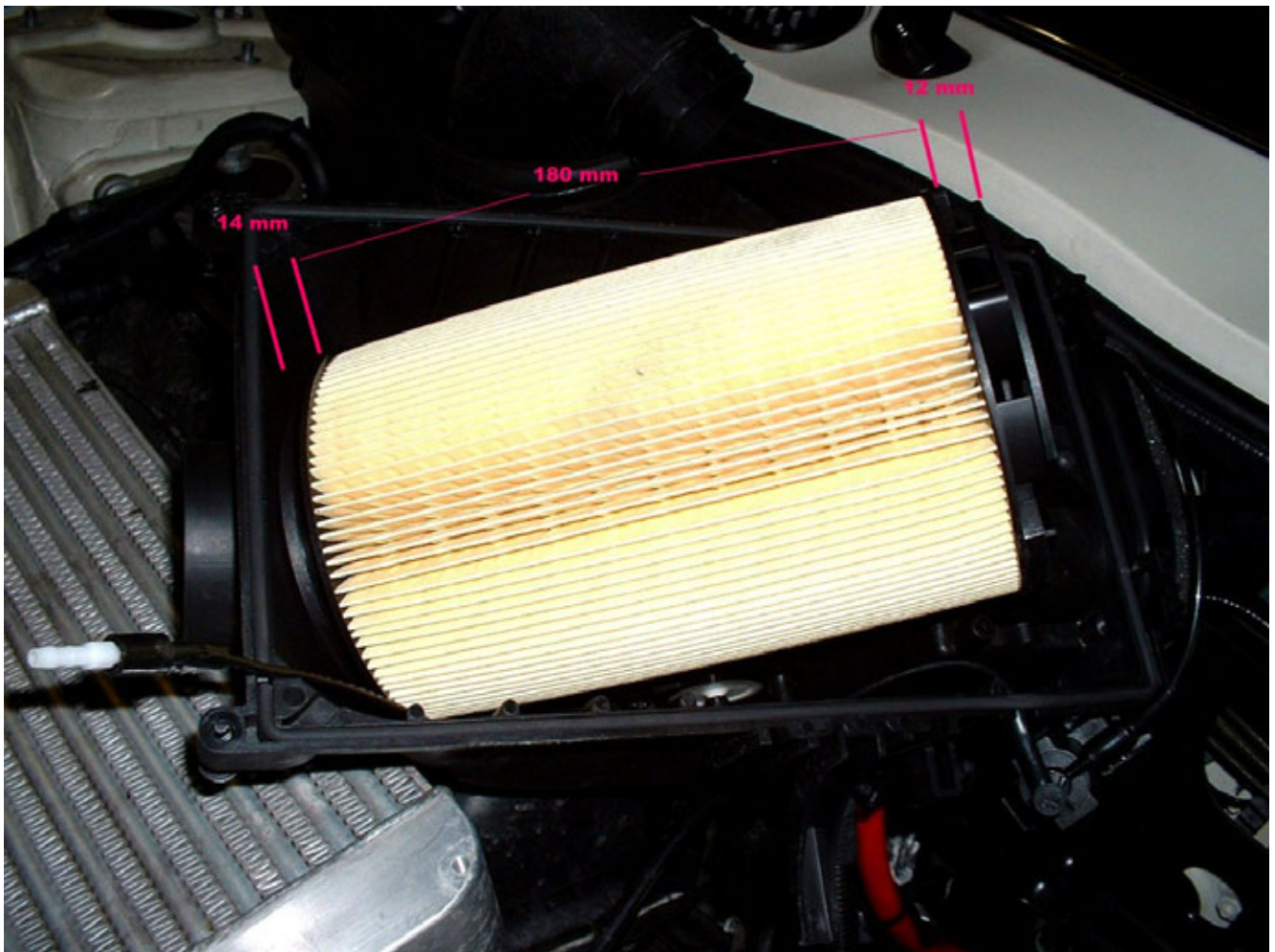
↑ Filter element fitted in upper part of filter housing
