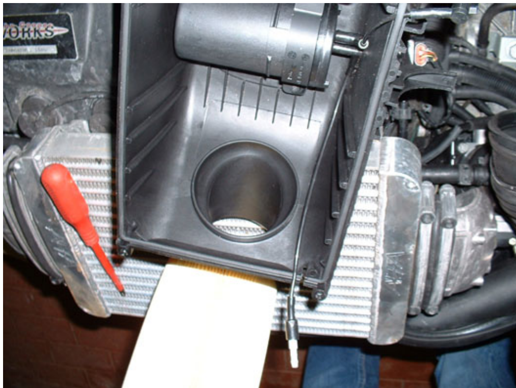
↑ upper part of filter housing, empty
